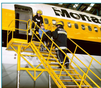
Aircraft Evacuation Chair
